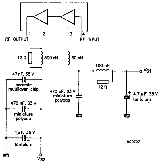
Fig.4 Decoupling arrangement.
